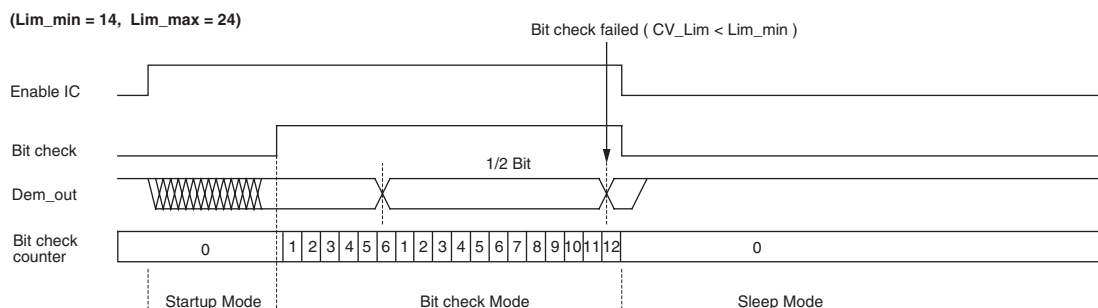
Figure 5-6. Timing Diagram for Failed Bit Check (Condition: \text{CV\_Lim} < \text{Lim\_min} )
